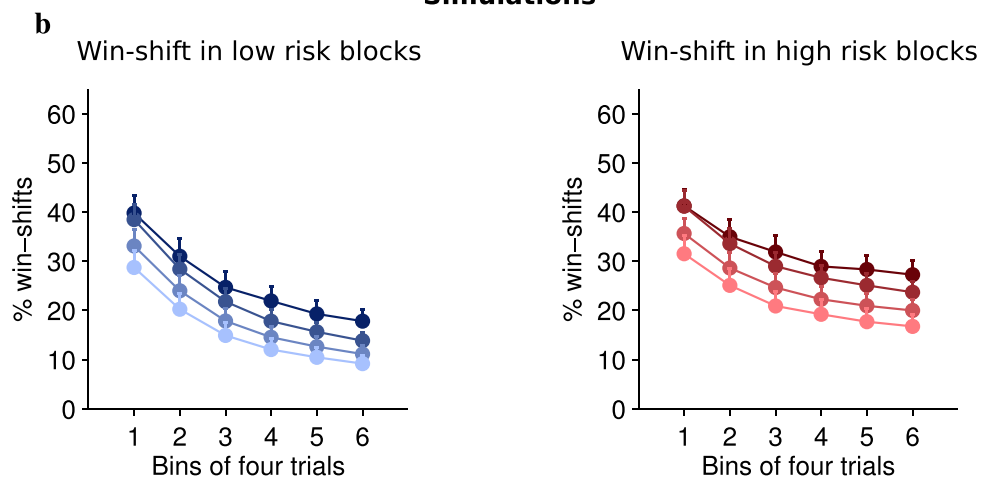
Figure 2. (a) Average proportion of win-shifts (mean + sem) of rats across a block as a function of risk and flupenthixol dose. (b) Average win-shift of model simulations.
